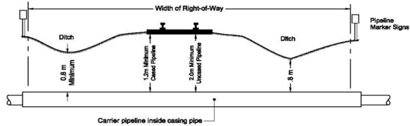
A Typical Railway Crossing
