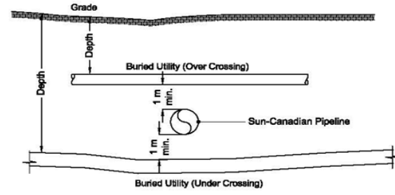
D Typical Utility Crossing
