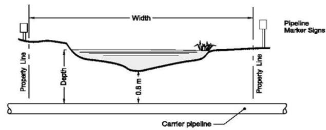
C Typical Ditch Crossing
