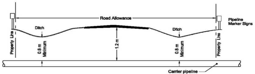
B Typical Road Crossing
